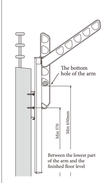
Side View of Railing and Laundry Pole Holder
