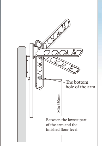
Side View of Railing and Laundry Pole Holder
