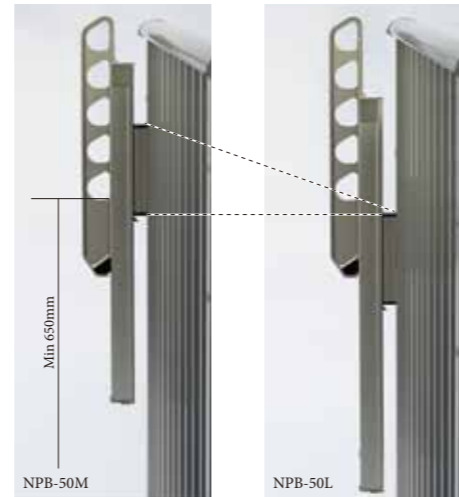
How to change the height of a pole holder
