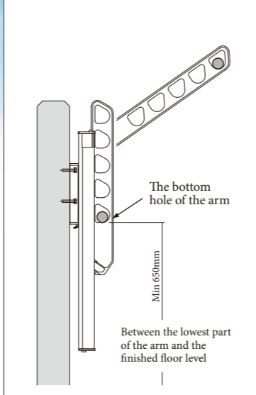
Side View of Railing and Laundry Pole Holder
